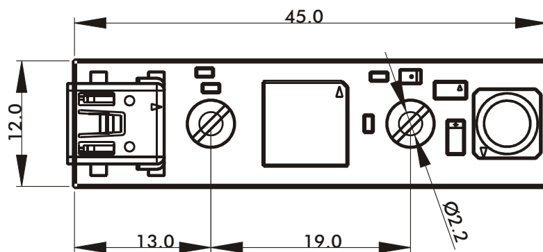
Figure 1: Mechanical dimensions of the Oak G sensor
