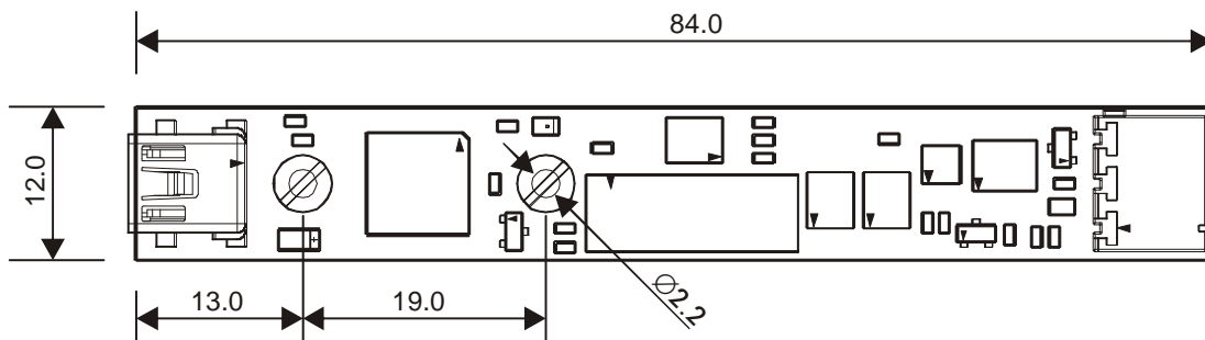
Figure: Mechanical dimensions of the Oak 4-20 sensor
